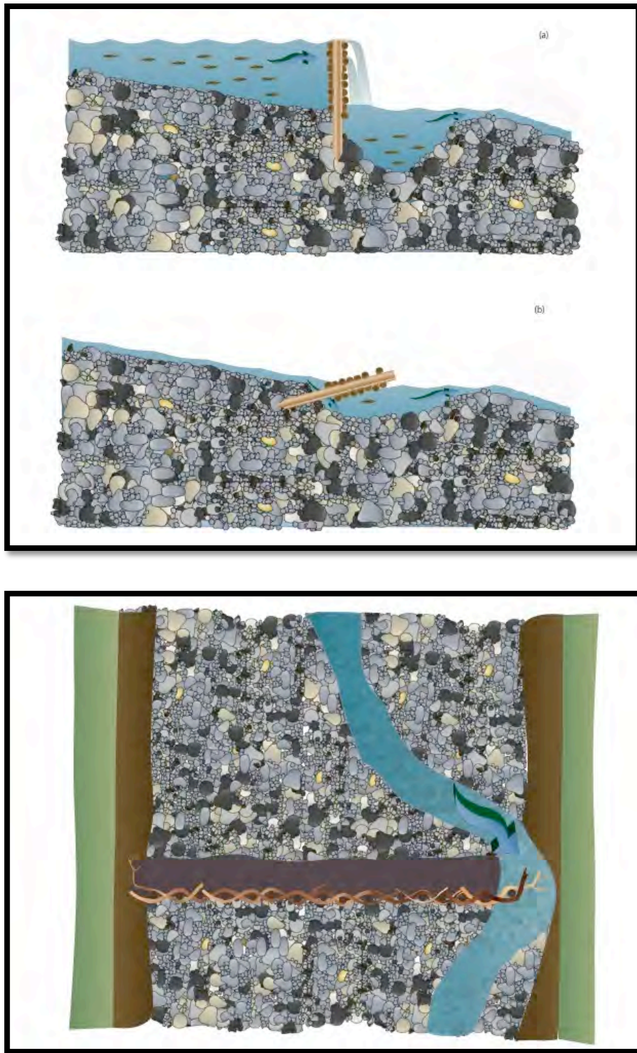
Figure 30: Examples of beaver dam analogue failure mechanisms: (top) overtopping downstream scour followed by underscour; posts that are not pounded deeply enough into the bed deep can be undermined by overtopping downstream scour, and (bottom) lateral scour of an erodible bank results in an end cut.
